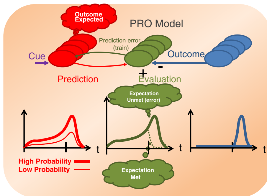
Fig. 1. A general conceptual illustration of the Predicted Response Outcome (PRO) model of anterior cingulate cortex. Left: The prediction units (red) generate a timed prediction of what outcomes are expected, with what probability, and when. There are four prediction units (ellipses) shown here for illustration purposes, corresponding to four predicted outcomes, although the number of prediction units will vary in general with different tasks so that there is one prediction unit for each corresponding possible outcome. Lower left: Greater probabilities (y-axis) are associated with greater prediction activity, which peaks at the time when the outcome is expected due to the temporal discounting of the probability. Middle: The evaluation units compute negative surprise , i.e. they detect when an expected outcome fails to occur. This is simply the difference between the predicted and actual outcomes and represents how improbable the negative surprise was. The green arc from evaluation to prediction indicates that prediction errors from the evaluation units train and update the prediction signals. Lower middle: Events that are predicted with a high probability yield greater surprise signals (expectation unmet) when they fail to occur, but a weaker surprise signal when they do occur (expectation met). Right: Outcomes occur (i.e. outcome value rises rapidly and transiently to 1) or fail to occur (i.e. outcome value is 0) at specific times.
