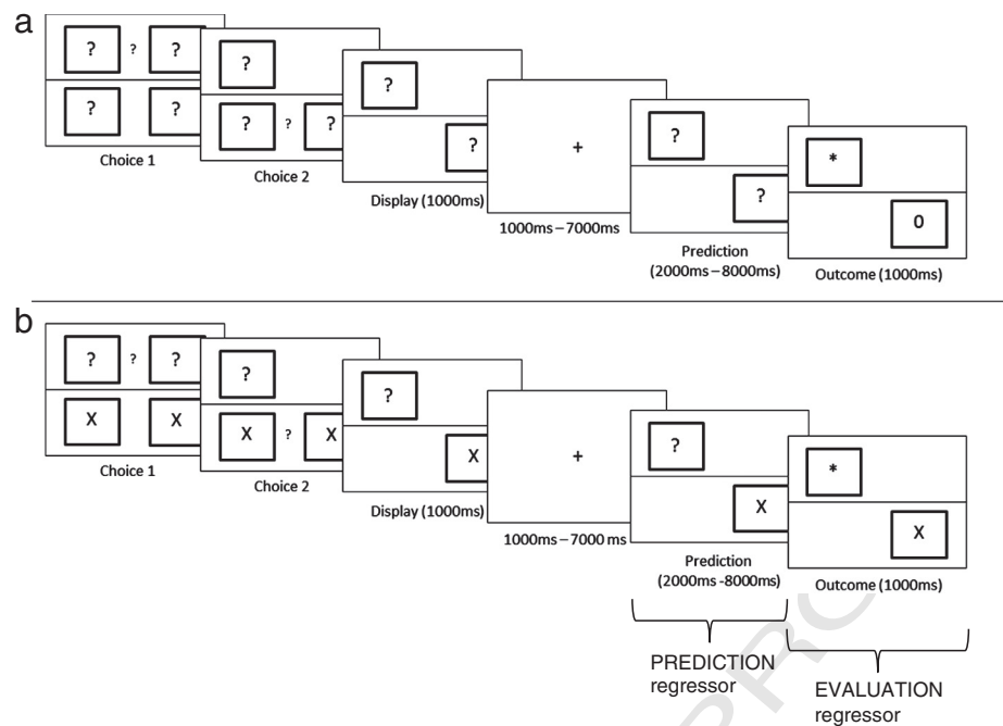
Fig. 2. Task design. Dissociation of decision, prediction, and outcome effects. In each trial, the question mark between the two upper or two lower boxes prompted a choice between the adjacent boxes. After a delay to separate out the decision and motor-related activities, subjects were re-presented with their choices, at which point they could predict the impending feedback to be delivered in the outcome phase of the trial. Outcomes (“*” and “0”) shown later in the chosen boxes indicated that subjects should choose the same box again on the next trial (stay) or, less commonly, choose a different box on the next trial (switch). (a) In the Predict2 condition, participants made a series of two choices and later received outcome feedback for each choice. During the prediction phase of the task, participants could predict the impending outcome(s). (b) In the Predict1 condition, participants also made two choices, but they knew that they would receive only a single outcome cue. No feedback was given for boxes containing an “X”. Instead, participants were told to repeat their previous choice in the next trial. Hence, there was only a single outcome to predict and evaluate in the Predict1 condition. Overall, the task affords distinct activity estimates of decisions, of predicting 1 vs. 2 outcomes, and of receiving 0, 1, or 2 rare switch feedback cues. The actual stimuli were shown to subjects with the colors inverted, i.e. white stimuli on black background.
