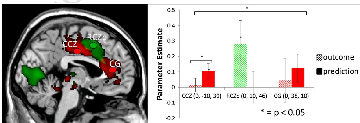
Fig. 3. Regions of the CCZ/ACC showing increased activation in response to prediction- and outcome-related effects as predicted by the PRO model, presented at a cluster corrected threshold of p < 0.05 . The RCZp and CG ROIs were taken from Nee et al. (2011), while the CCZ ROI was created from coordinates reported in Drabant et al. (2011). Red: Prediction-related effects; green: Outcome-related effects.
