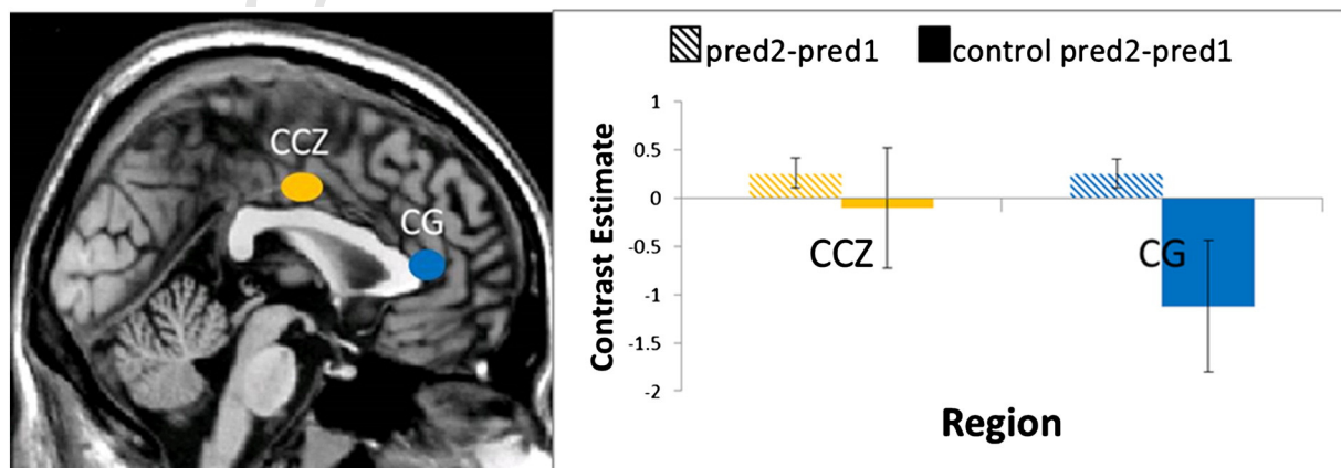
Fig. 4. Regions of the posterior cingulate (CCZ) and anterior cingulate (CG) showing increased activation for predicting 2 outcomes (Predict2) as opposed to predicting 1 outcome (Predict1). Within these independent ROIs, parameter estimates were extracted for the control condition. A paired t-test in both regions revealed that the parameter estimates for the Predict2–Predict1 contrast were significantly greater than for the control contrast. The control condition did not pass any corrected thresholds in a whole-brain analysis.
