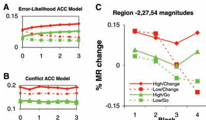
Fig. 3. Learning effects across time. (A) The error-likelihood computational model with adaptive ACC inputs predicts an initial effect of change > go and a subsequently growing effect of high > low in each of the change and go conditions. (B) The conflict computational model with fixed ACC inputs predicts an effect of high/change > low/change and change > go but no effect of high/go > low/go. None of these effects varied with time. MR, magnetic resonance. (C) fMRI results are consistent with the error-likelihood but not the conflict ACC model. During the first two blocks, activity in the anterior pre-SMA region shows effects of change > go but not of high > low, despite the fact that CSDs have equilibrated by the beginning of the second block (fig. S1). By the third and fourth blocks, both the change and go conditions show evidence of discrimination between high- and low-error conditions, and this discrimination eventually dominates the discrimination between change and go trials by the end of the session.
